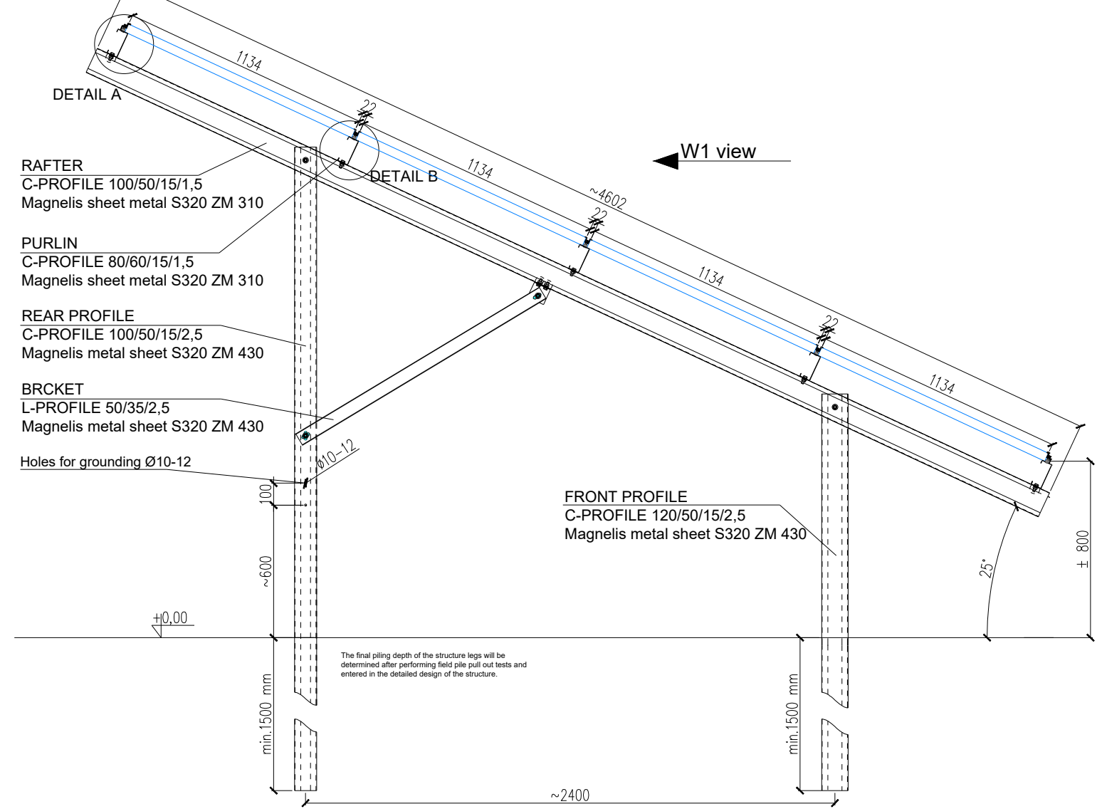
CROSS-SECTION A-A
