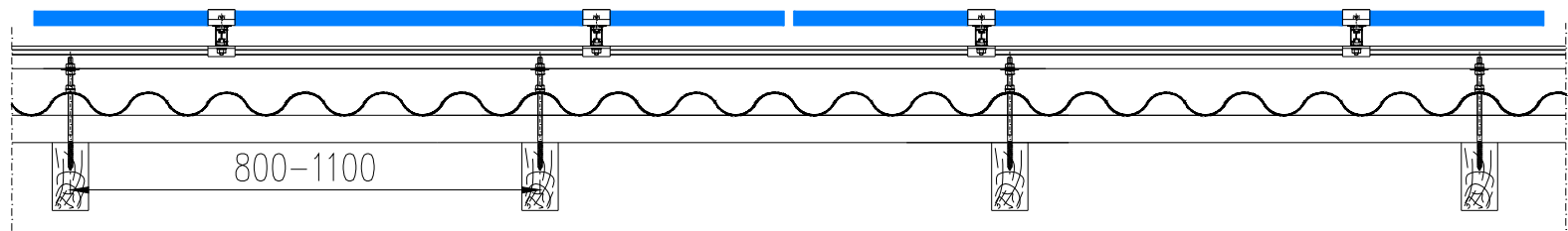
cross-section B-B
