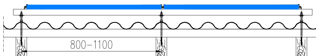
cross-section A-A
